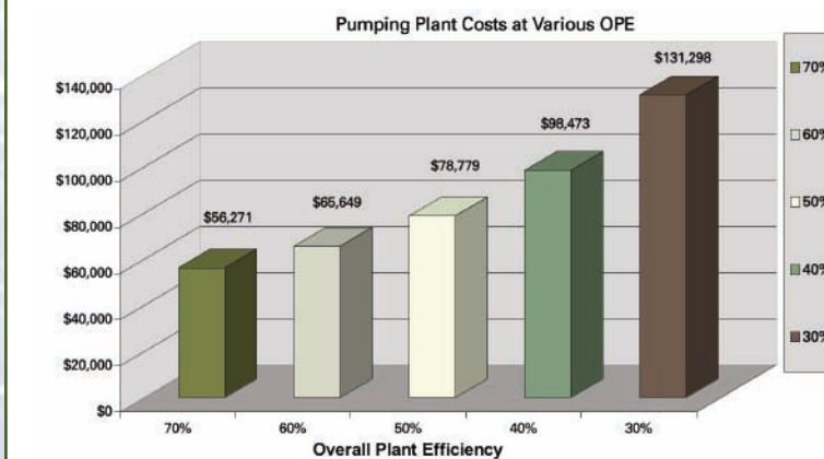
Example of cost to pump 1,000 Acre Feet at 300 Total Head and $.11/kWh
